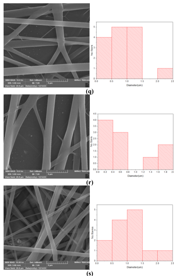
Fig. (9) SEM images of PVP (16, 17, 18 and 19) at different collector rotation speeds as shown in table (1) at 5 \mu m scale
