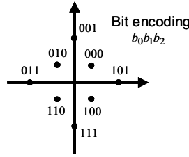
Fig. 9. 8-QAM constellation.
