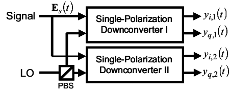
Fig. 7. Dual-polarization downconverter.
