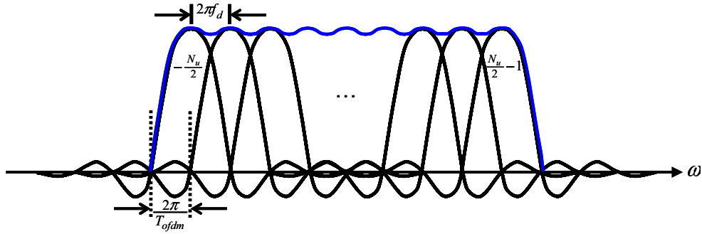
Fig. 23. Spectrum of OFDM signal.
