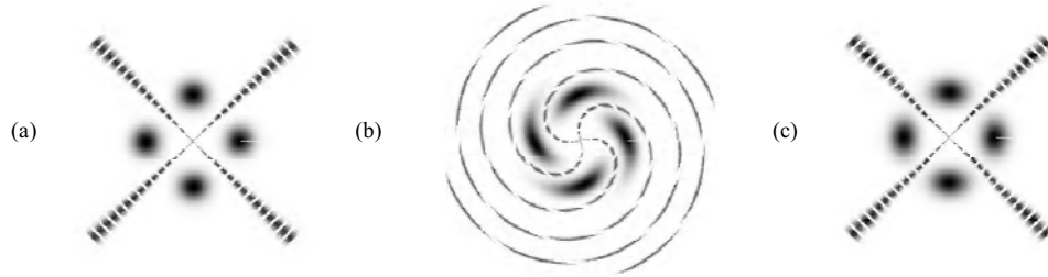
Fig. 15. Constellation diagrams of the received signal showing ML decision boundaries for (a) no NLPN, (b) with NLPN before compensation by \theta_{opt} , and (c) with NLPN after compensation by \theta_{opt} .
