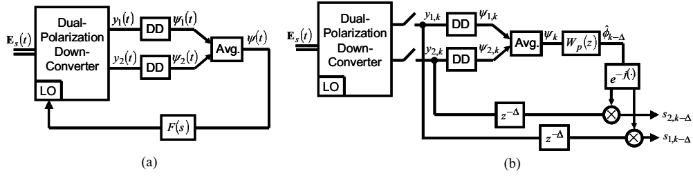
Fig. 19. Carrier synchronization for polarization-multiplexed systems, (a) PLL approach, (b) feedforward carrier synchronization approach.
