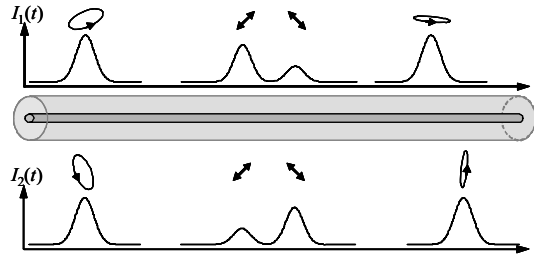
Fig. 11. First-order polarization-mode dispersion.
