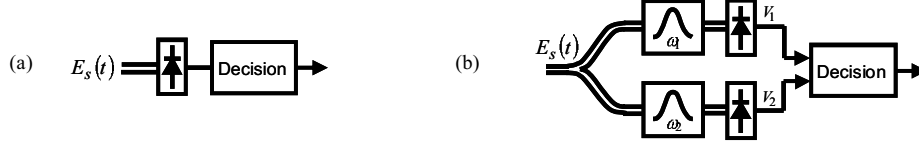
Fig. 1. Noncoherent receivers for (a) amplitude-shift modulation (ASK) and (b) binary frequency-shift keying (FSK).
