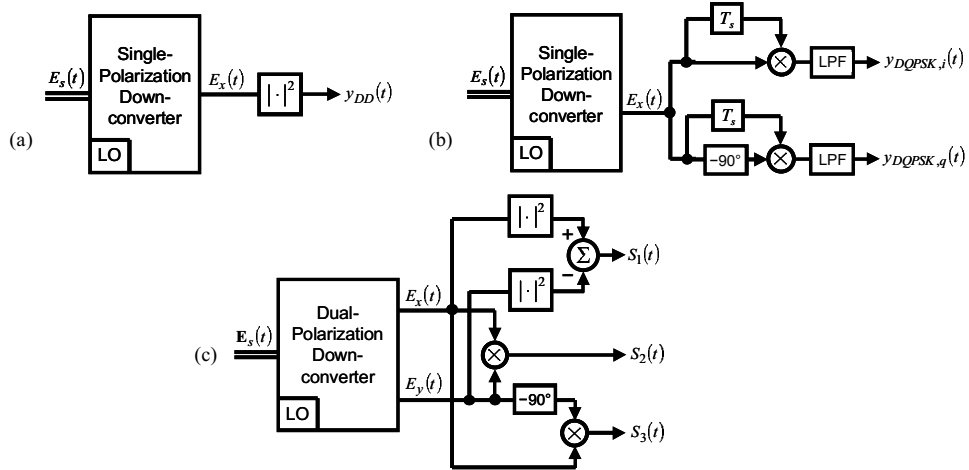
Fig. 8. Emulating (a) direct detection, (b) 4-DPSK detection and (c) PolSK detection with optoelectronic downconversion followed by non-linear signal processing in the electronic domain. The signals E_x(t) and E_y(t) are the complex-valued analog outputs described by Eq. (12) for each polarization. We note that in the case of the heterodyne downconverter, the non-linear operations shown can be performed at the IF output(s) of the balanced photoreceiver.
