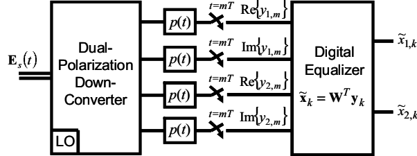
Fig. 12. Digital equalization for a dually polarized linear channel.
