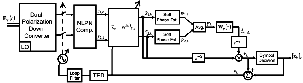
Fig. 20. Integration of adaptive digital equalization with carrier synchronization.
