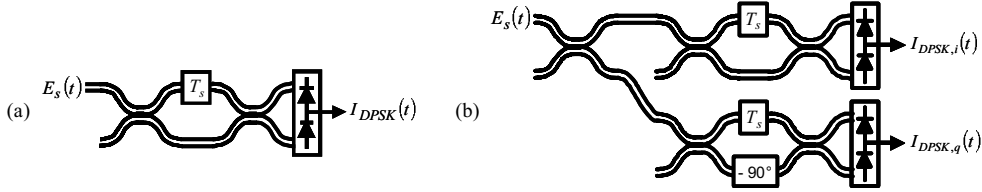
Fig. 2. Differentially coherent phase detection of (a) 2-DPSK (b) M -DPSK, M > 2 .
