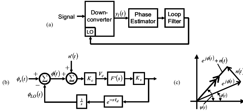
Fig. 16. Phase-locked loop: (a) System model, (b) analytical model, (c) phase estimation.
