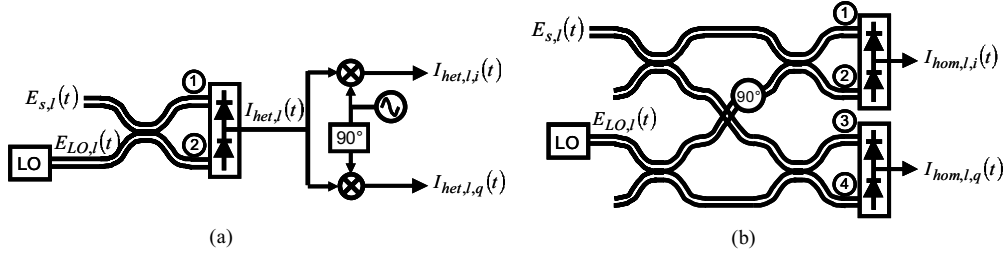
Fig. 5. Single-polarization downconverter employing a (a) heterodyne and (b) homodyne design.
