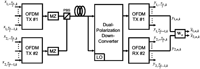
Fig. 24. Polarization-multiplexed OFDM transmitter and receiver with PMD compensation.
