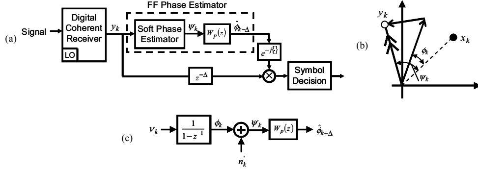
Fig. 18. Feedforward carrier phase estimation. (a) System model, (b) soft phase estimation, (c) analytical model.
