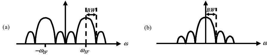
Fig. 6. Spectrum of a (a) heterodyne and (b) homodyne downconverter measured at the output of the balanced photodetector.
