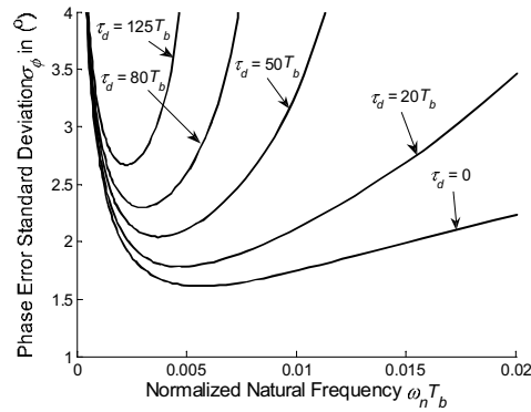
Fig. 17. \sigma_\phi versus \omega_n for 16-QAM at 100 Gbit/s in a single-polarization employing a second-order PLL, with \Delta\nu = 100 kHz and an OSNR of 11.5 dB.
