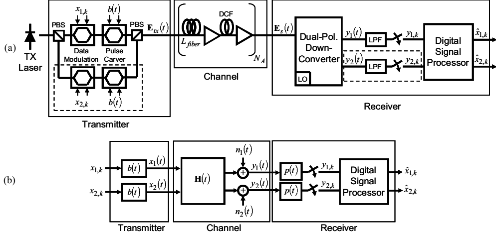
Fig. 4. Coherent transmission system (a) implementation, (b) system model.
