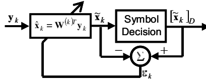
Fig. 13. Adaptive equalizer for polarization-multiplexed coherent detection.
