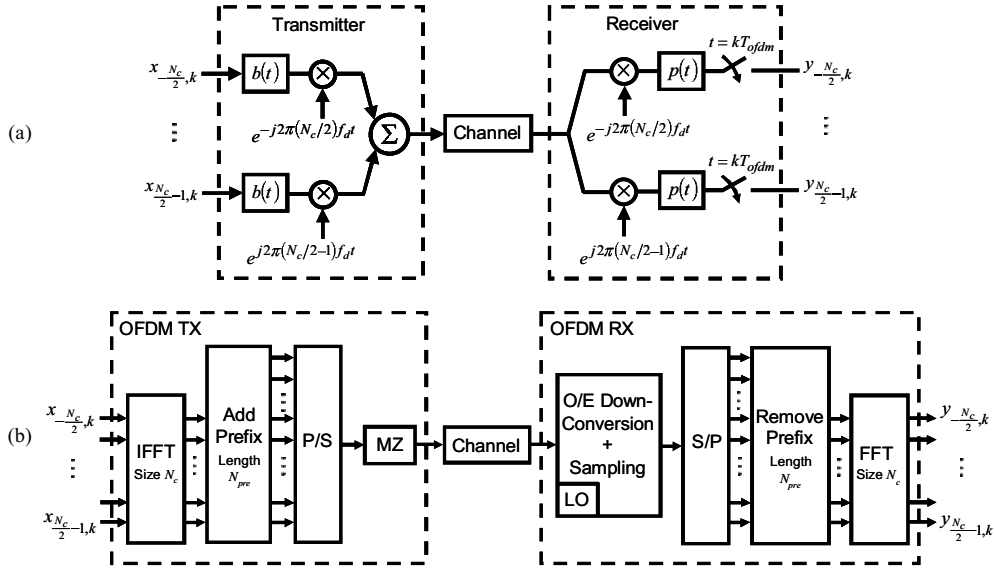
Fig. 21. Multi-carrier transmitter and receiver (a) analog implementation, (b) OFDM implementation.
