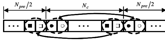
Fig. 22. OFDM symbol with cyclic prefix.
