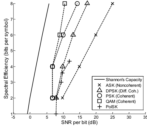
Fig. 10. Spectral efficiency vs. SNR per bit required for different modulation formats at a target BER of 10^{-3} . We assume polarization multiplexing for all schemes except PolSK. Also shown is the Shannon limit (15), which corresponds to zero BER.
