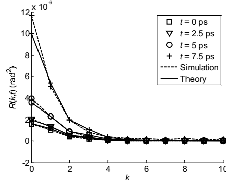
Fig. 14. Autocorrelation function for IFWM phase noise in 80 Gbit/s QPSK transmission with 33% Gaussian pulses. Each span consists of 80 km of SMF with \alpha = 0.25 dB/km, D = 17 ps/nm-km, \gamma = 1.2 W -1 km -1 , followed by DCF with \alpha = 0.6 dB/km, D = -85 ps/nm-km, \gamma = 5.3 W -1 km -1 . The mean nonlinear phase shift is \Phi_{NL} = 0.0215 rad/span.
